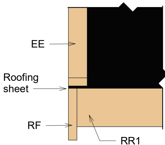
3 Roof Reinforcement
