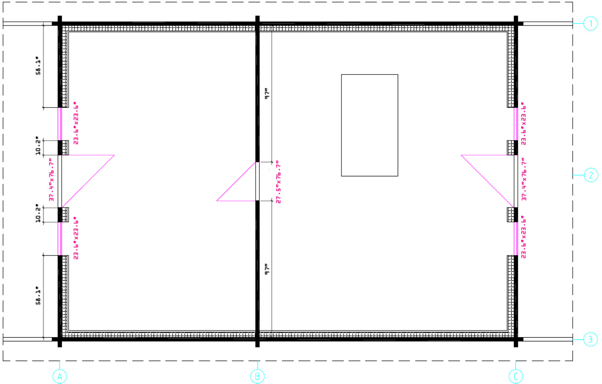
MUSKOKA // 70 / 18 - SECOND FLOOR
