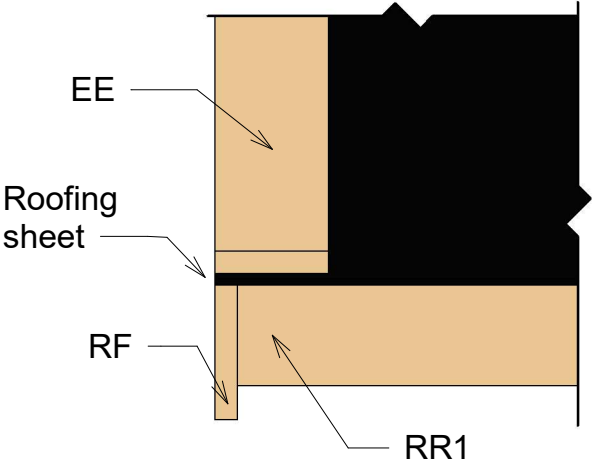
(3) Roof Reinforcement
