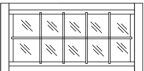
Window 765x1565
