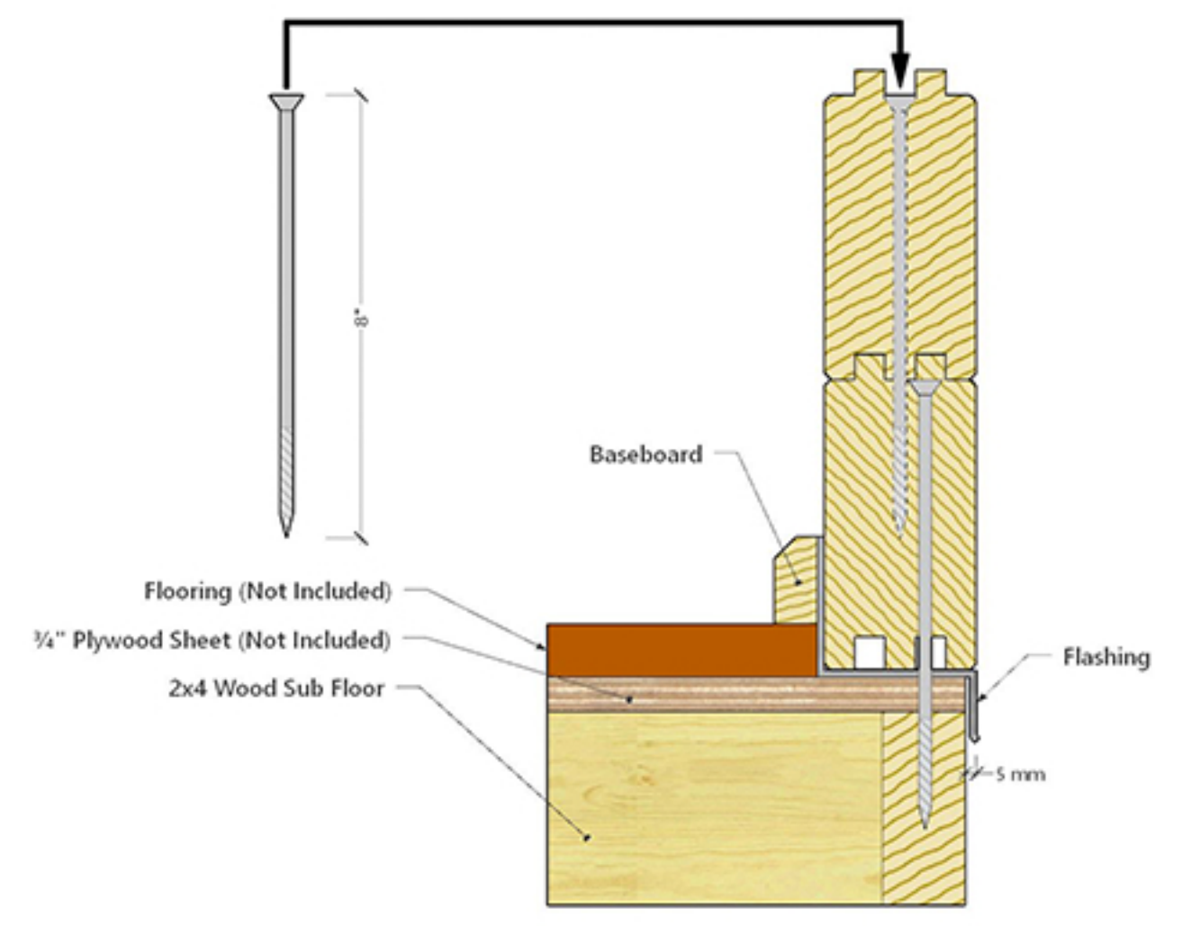
Foundation Connection Sub Floor
