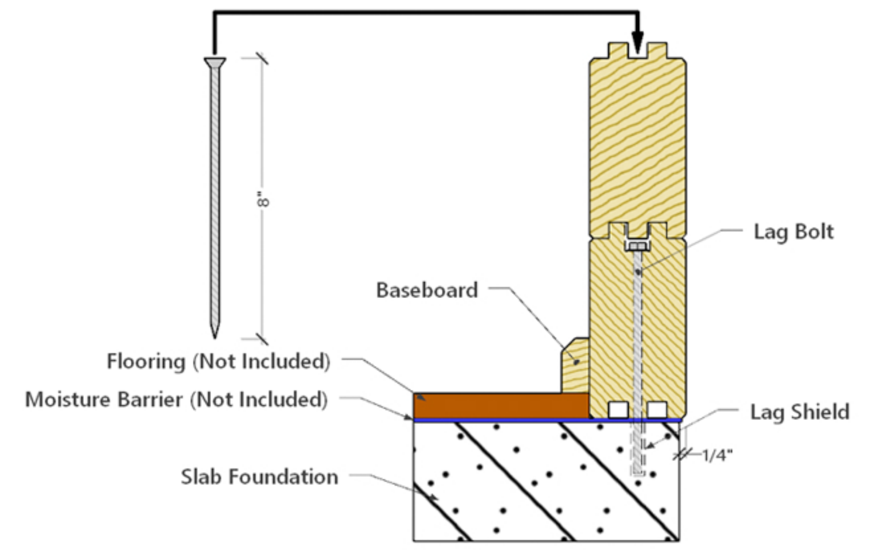
Foundation Connection Slab
