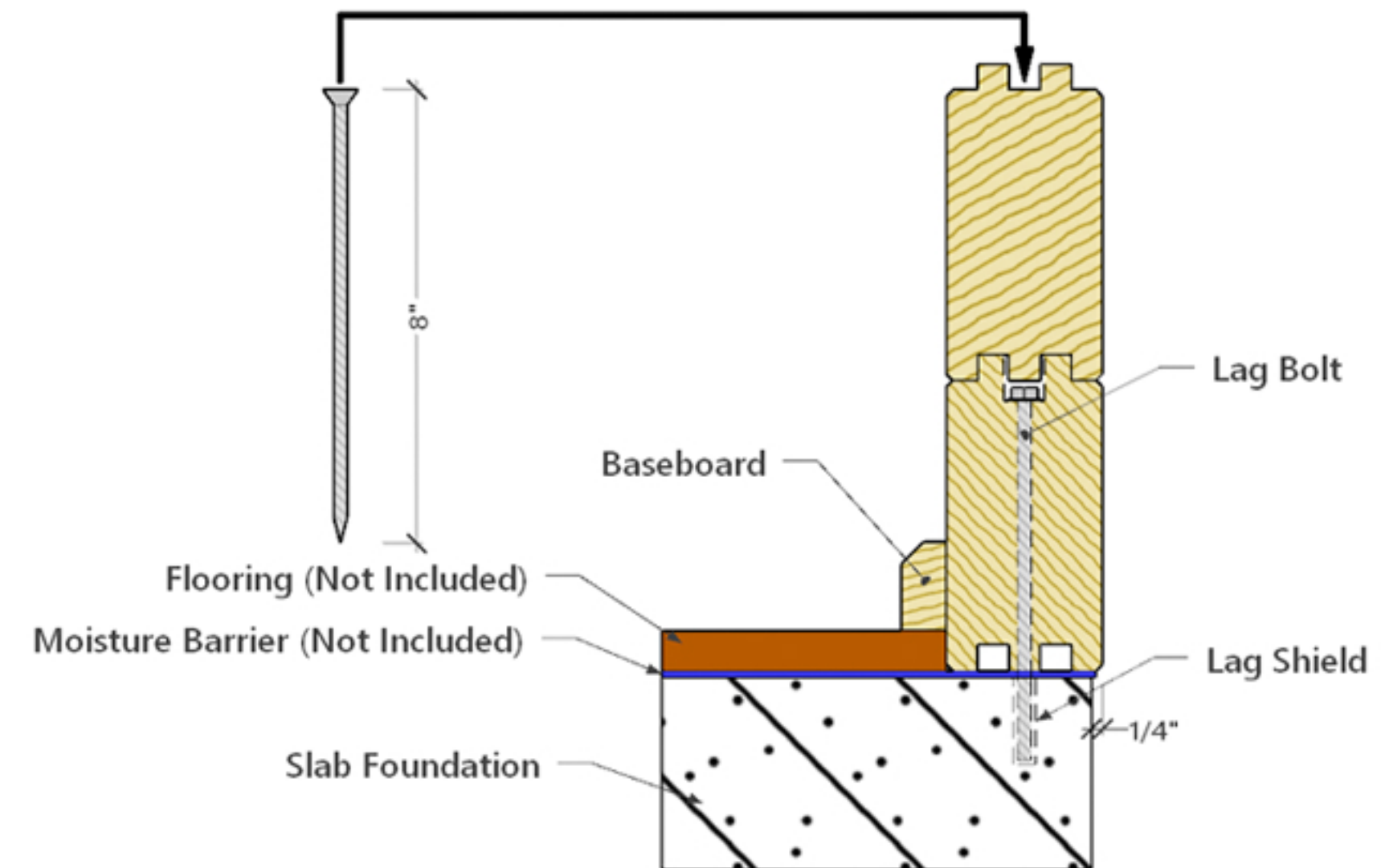
Foundation Connection Slab
