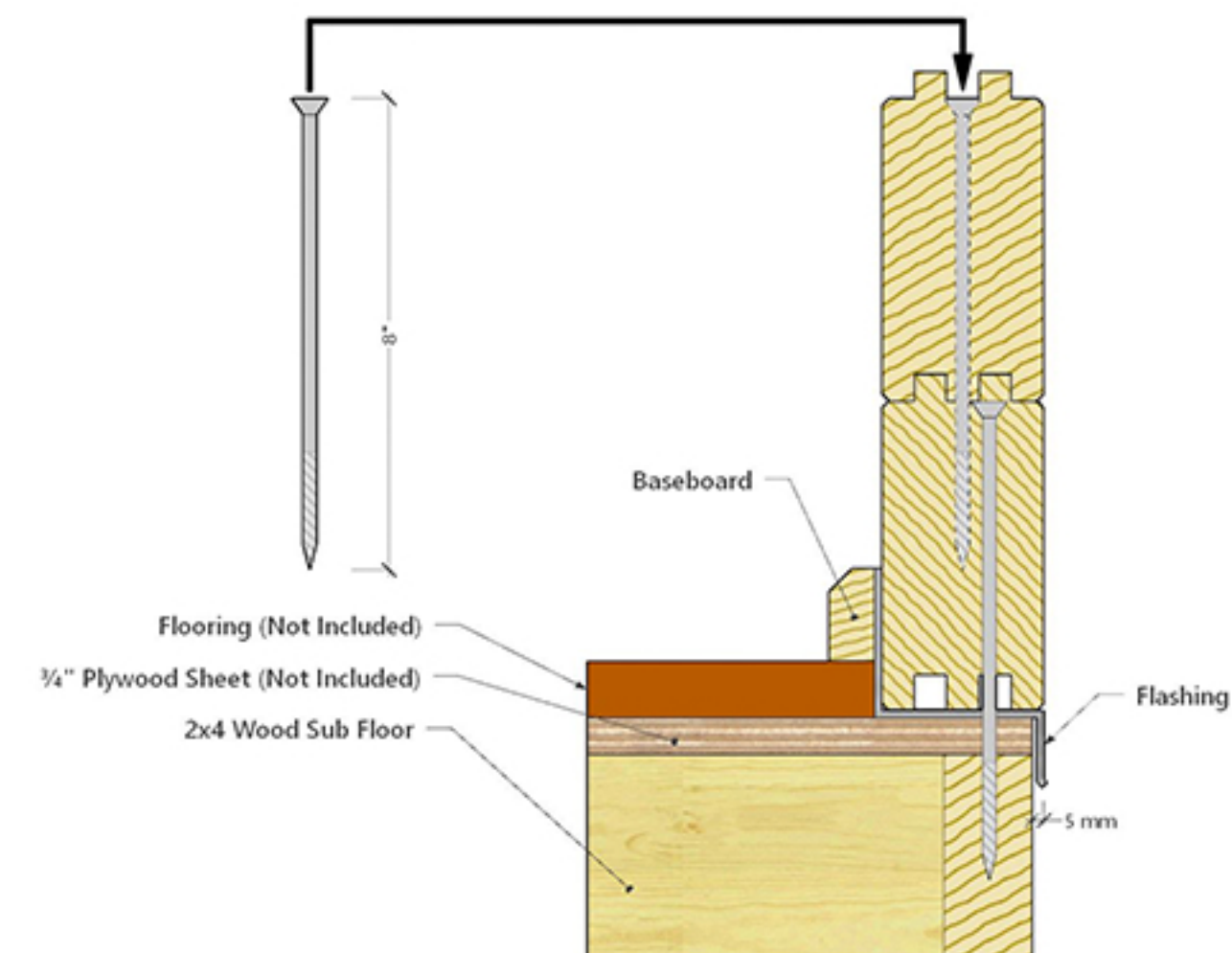
Foundation Connection Sub Floor
