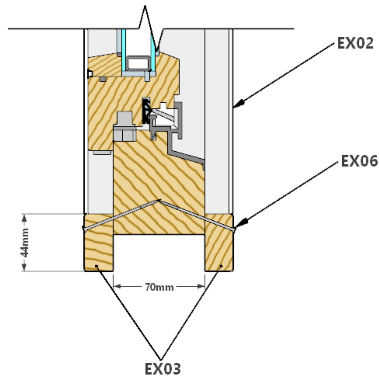
Window Section Detail
