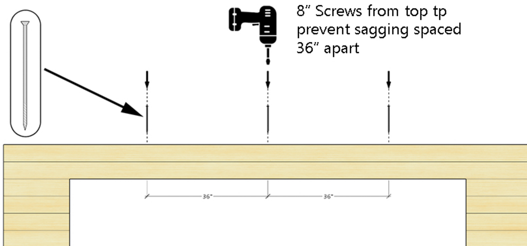
Stacked Beams Over Large Spans
