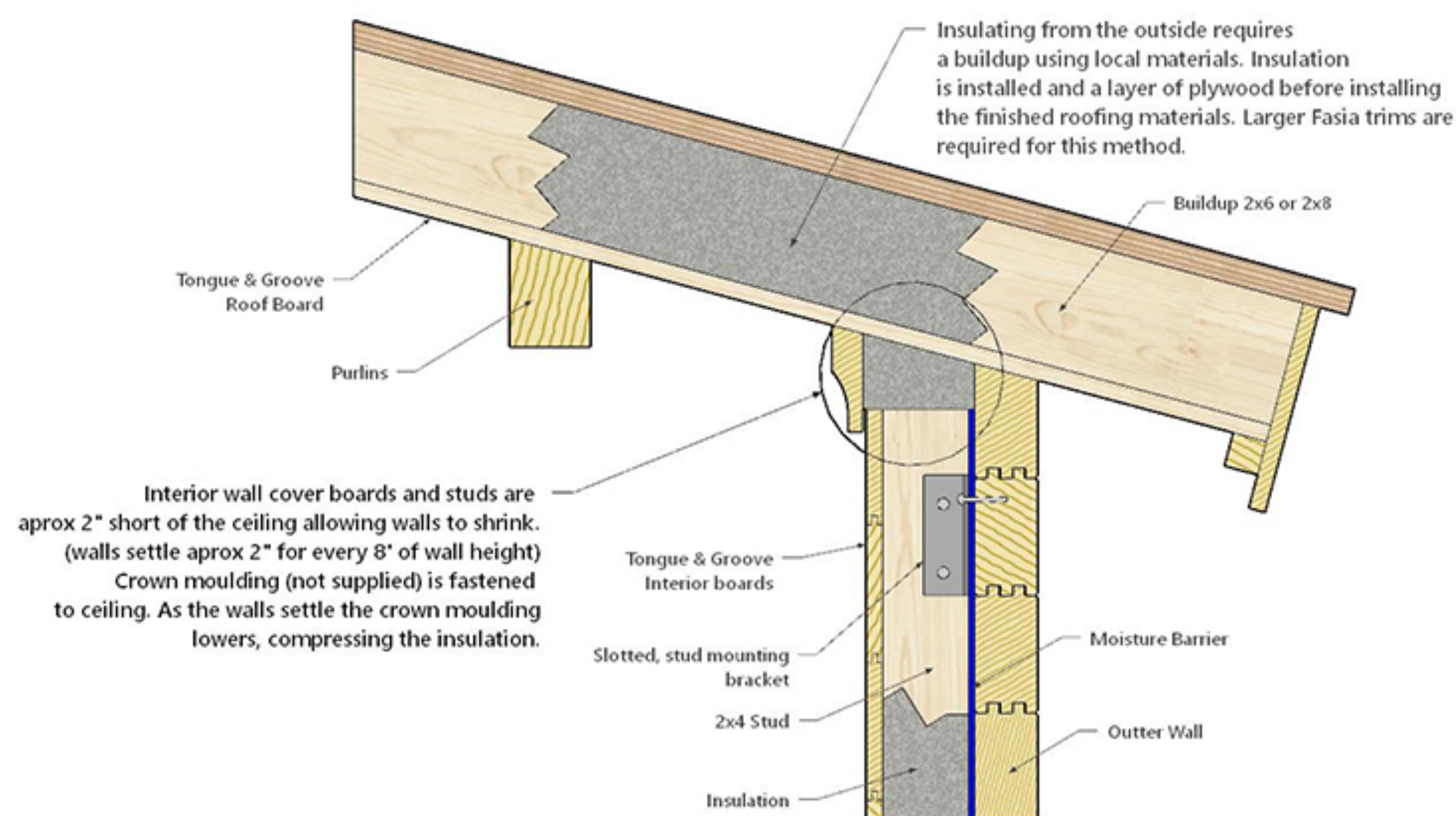
Exterior Roof & Interior Wall Insulation
