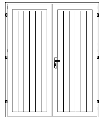
Nr. 13 Double door 56 1/8" x 69 7/8" 1 1/8"
