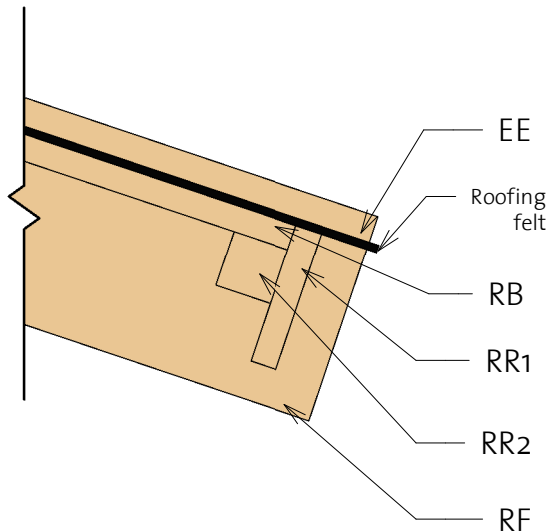
3 Roof Reinforcement
