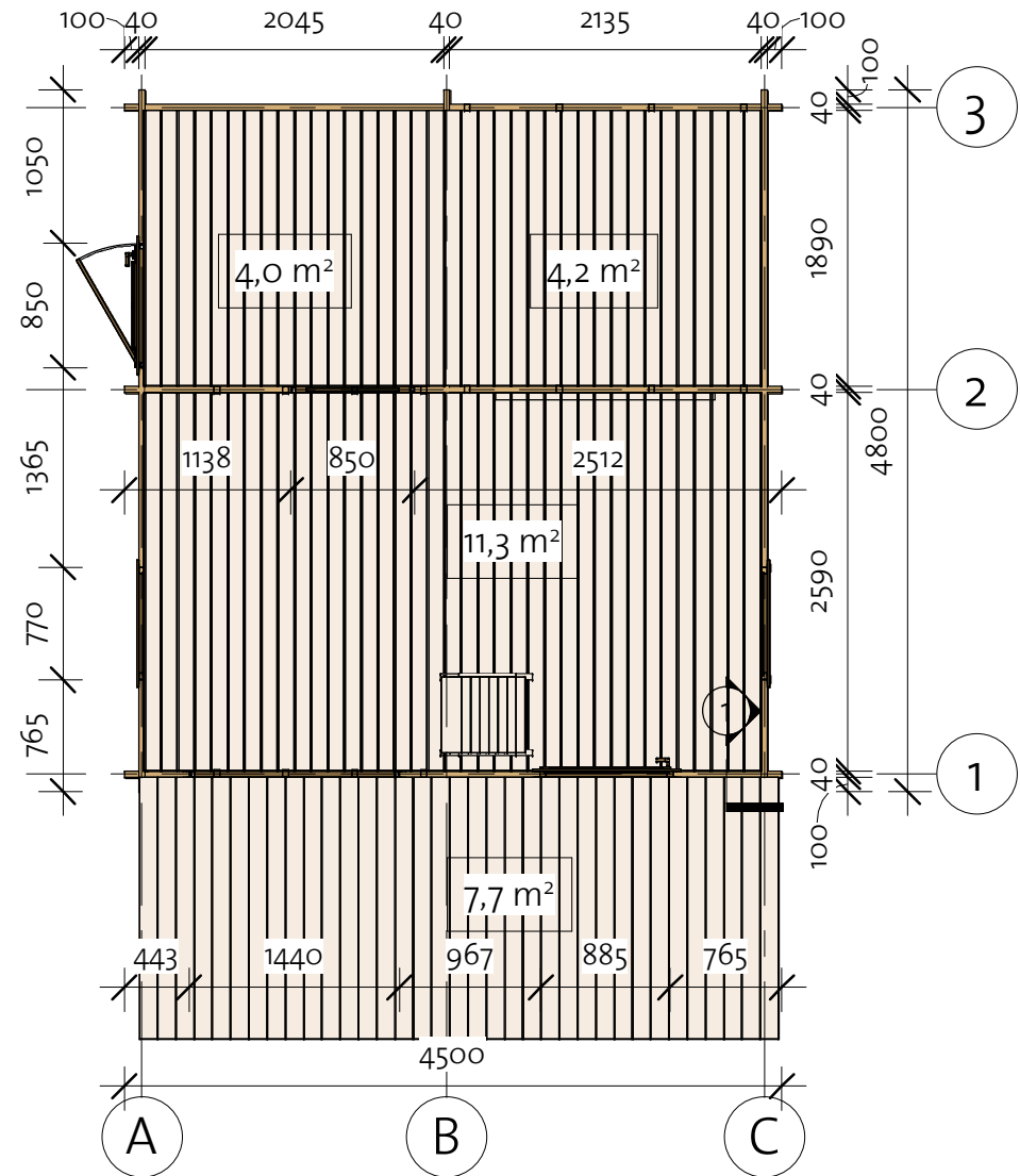
Sauna schedule
