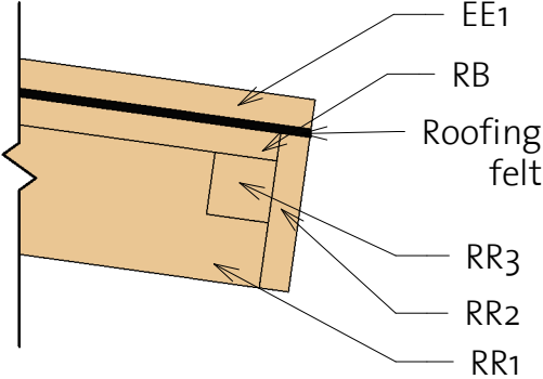
2 Roof Reinforcement 1
