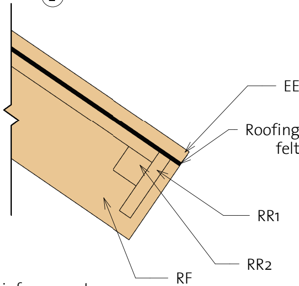
③ Roof Reinforcement
