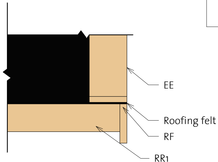
③ Roof Reinforcement
